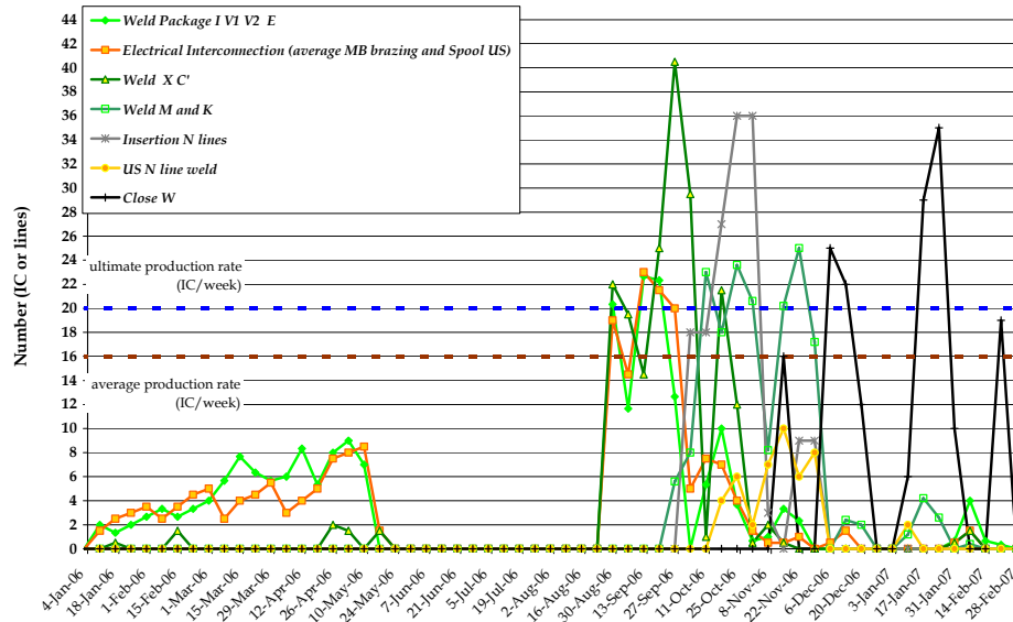
Fig. 5: Production rates in sector 4-5.
