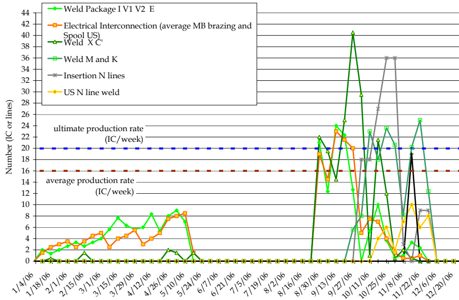
Fig. 3: Production rates in sector 4-5.
